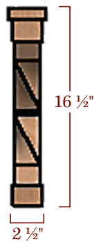
Side View 3"
